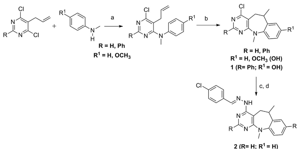
Scheme 1. Synthesis of 4-chloro-6,11-dimethyl-6,11-dihydro-8-hydroxy-2-phenyl-5H-benzo[b]pyrimido[5,4-f]azepine, ( 1 ) ( R = \text{Ph} ; R^1 = \text{OH} ) [49] and ( E )-4-(2-(4-chlorobenzylidene)hydrazinyl)-6,11-dimethyl-6,11-dihydro-5H-benzo[b]pyrimido[5,4-f]azepine ( 2 ) ( R = R^1 = \text{H} ).
