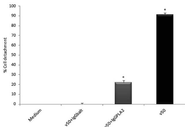
Fig. 5. Endothelial cell detaching activity of Bothrops alternatus venom after selective neutralization of either SVMP or PLA 2 with their corresponding specific antibodies. Cells were exposed for 3 h to venom alone (50 µg/mL; V50) or venom that was previously incubated with anti-baltergin IgG (IgGbalt) or anti-PLA 2 IgG (IgGPLA 2 ) at an antibody:venom ratio of 25:1 (w/w). Cell detachment was determined by crystal violet cell uptake assay, as described in Materials and methods . Readings from cells incubated with medium alone were considered as 0% detachment (100% attachment). Each bar represents mean ± SD of triplicate assays. Asterisks indicate a statistically significant ( p < 0.05 ) difference in comparison to controls.
