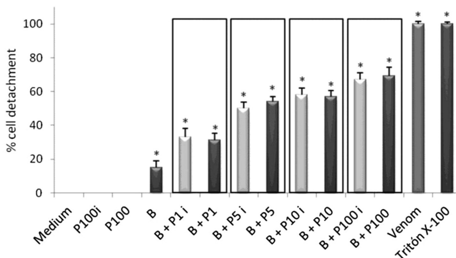
Fig. 4. Synergistic effect is independent of PLA 2 catalytic activity. Cells were exposed for 3 h with either Baltergin (B: 100 µg/mL, total volume: 200 µL) or a combination of Baltergin and catalytic active PLA 2 (B + P, Baltergin 100 µg/mL and PLA 2 1–100 µg/mL, total volume: 200 µL) or Baltergin and catalytic inactive PLA 2 (B + Pi: Baltergin 100 µg/mL and PLA 2 i 1–100 µg/mL, total volume: 200 µL). Bothrops alternatus venom (100 µg/mL, total volume: 200 µL) and 0.1% Triton X-100 were used as positive controls of detachment; culture medium was used as negative control. Cell detachment was determined by crystal violet uptake, as described in Materials and methods . Each bar represents mean ± SD of triplicate assays. (*) indicate a statistically significant ( p < 0.05 ) difference in comparison to untreated cells.
